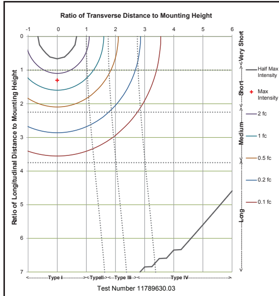
ISO FootCandle Plot at 4 Feet
