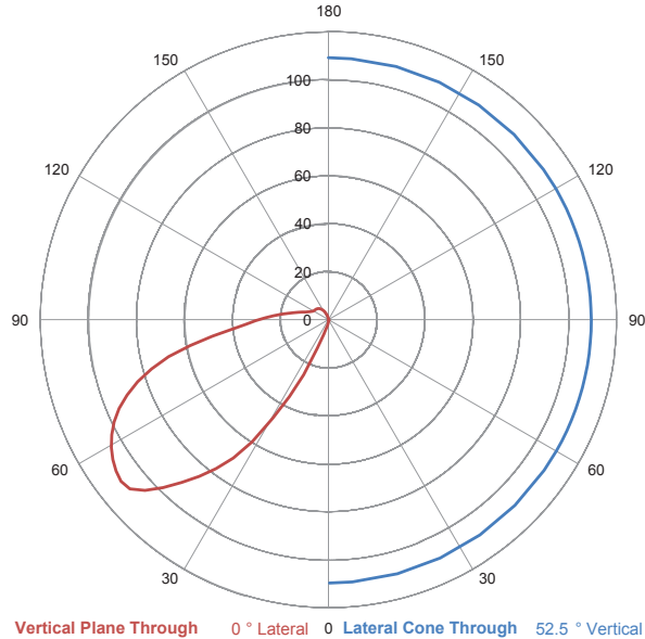
Maximum Plane and Cone Plots of Candela
