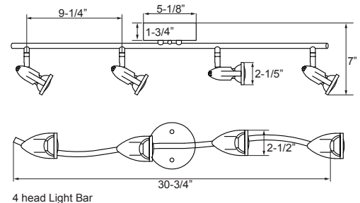
4 head Light Bar
