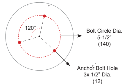
180SH Shield Rear View
