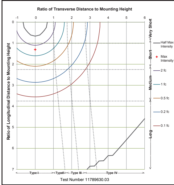
ISO FootCandle Plot at 4 Feet
