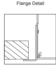
Exposed Flange Detail: Specify FT in part #
